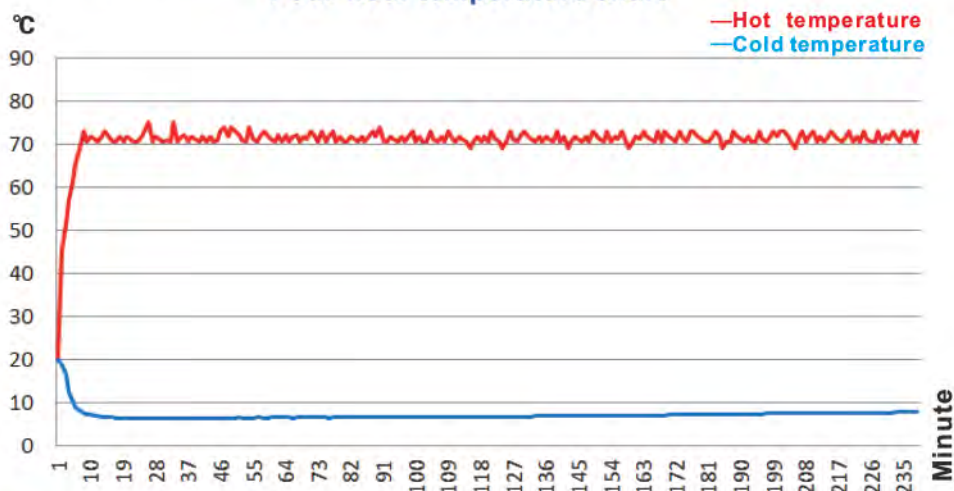
Four-hour temperature chart
